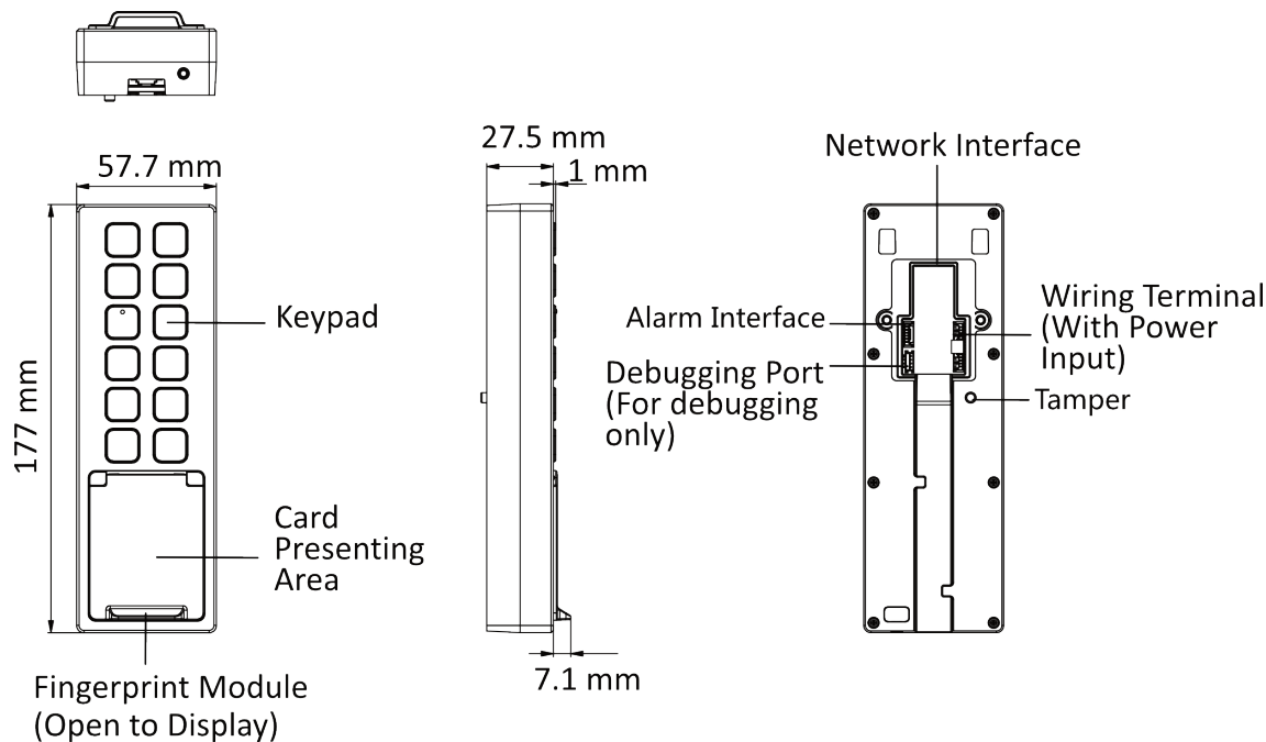
Figure 2-1 Access Control Terminal (Fingerprint + Card Series)
