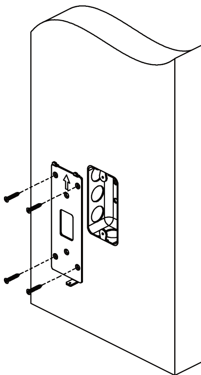
Figure 3-8 Install Mounting Plate
